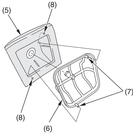
(5) air cleaner (6) air cleaner holder (7) tabs (8) holes
